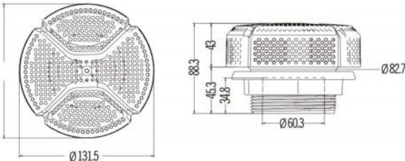
L-3901 2" Found Suction Black
