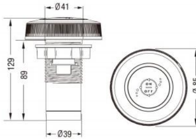
L-7042C 1" Honor Air Controls
