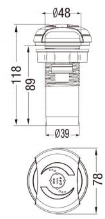
L-2213C 1" Wei Navigation Air Control Transparent
