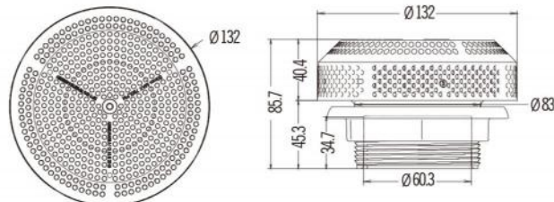
L-3802B 2" Soar Suction Black
