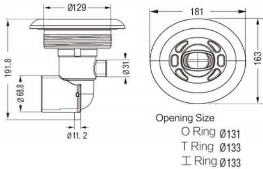
L-2805S 7.5" Oval Jet Black
