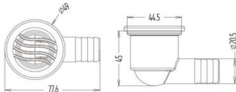
L-3808 Spa Floor Drain
