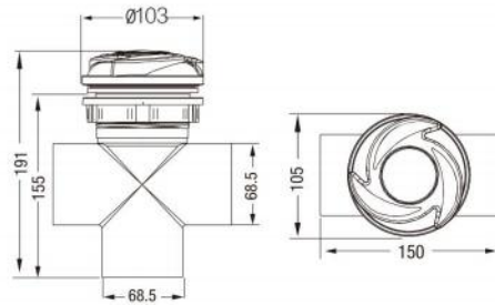
L-2027S 2" Xiong Feng Diverter Valve (SS Cover) Black
