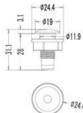
L-2304 1/2" threaded Light Lens
