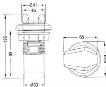
L-2041C 1" Found Air Controls Transparent
