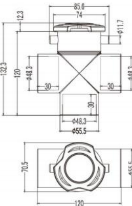
L-2046 1.5" Handsome Elegant Diverter Valve Black
