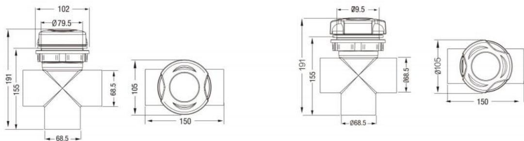
L-2030 2" Handsome Elegant Diverter Valve Black L-2030C 2" Handsome Elegant Diverter Valve Transparent L-2030S 2" Handsome Elegant Diverter Valve (SS Cover)Black
