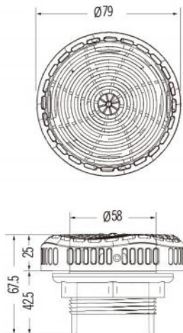
L-3806G 1.5" Cyclone Suction Grey
