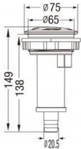
L-2202S 3.5" Ajar Water Feature (SS Cover)
