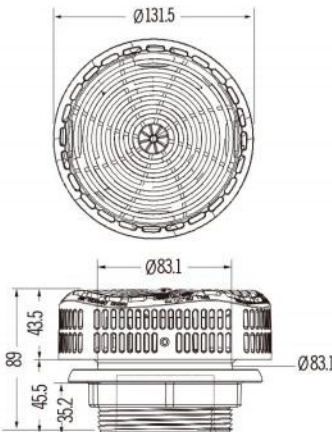
L-3807G 2" Cyclone Suction Grey
