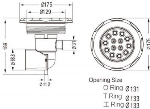
L-6705S 7.5" Elegant Multi-Massage Jet Black
