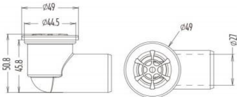
L-3809S SS Spa Floor Drain Black
