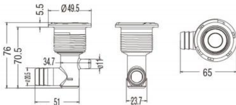
L-0247 2" Jet Body 3/4"RB × 3/8"SB
