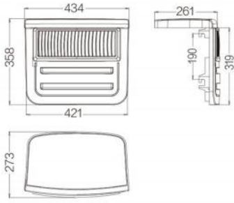
L-2173AB Grid Filter Black
