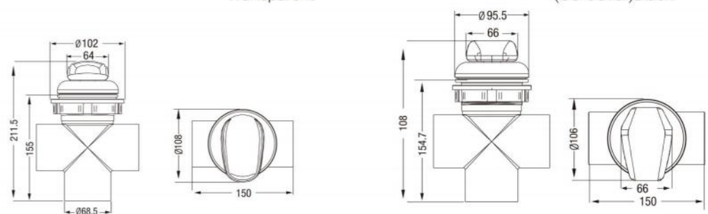
L-2043 2" Found Diverter Valve Black L-2043C 2" Found Diverter Valve Transparent L-2043S 2" Found Diverter Valve (SS Cover)Black
