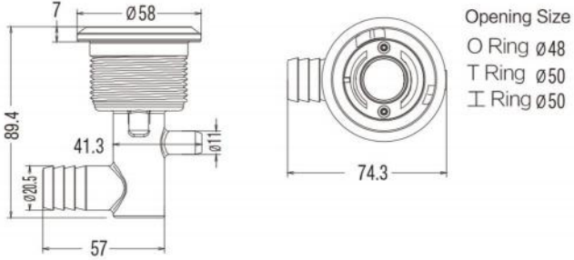
L-0077 2.5" Jet Body 3/4"RB × 3/8"SB
