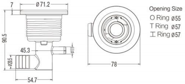
L-0432 3" Jet Body 3/4"RB × 3/8"SB
