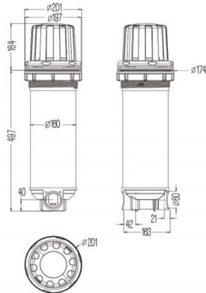
L-2137 Teleweir Skim Filter With Protective Cover
