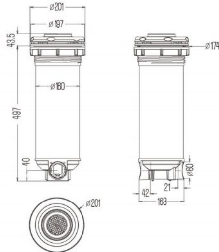
L-2136 Teleweir Skim Filter
