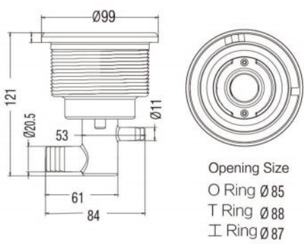
L-0144 4.5" Jet Body 3/4"RB × 3/8"SB
