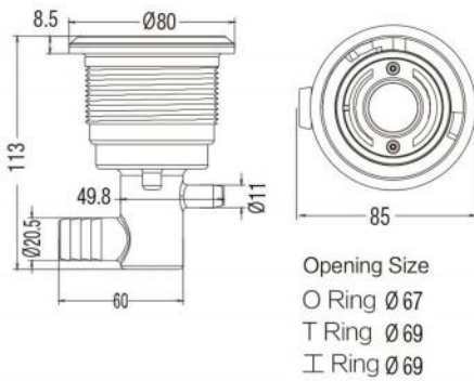
L-0120 3.5" Jet Body 3/4"RB × 3/8"SB
