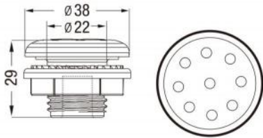
L-1114S 3/8" 9 Holes Air Jet Black
