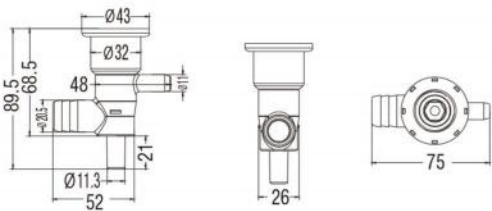
L-0008 1" Jet Body 3/4"RB × 3/8"SB
