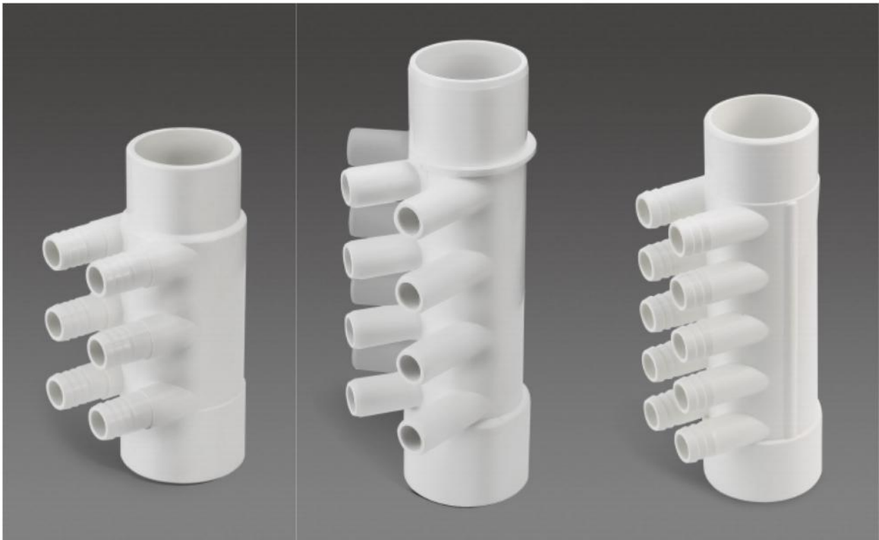
L-3002 2" 6 Holes Water Manifolds L-3039 2" 12 Holes Water Manifolds L-3009 2" 10 Holes Water Manifolds
