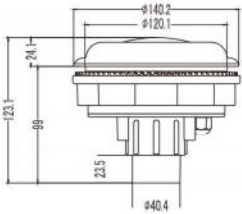
L-2010 Mushroom Waterfall Transparent
