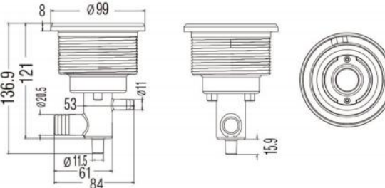
L-0258 4.5" Jet Body 3/4"RB × 3/8"SB
