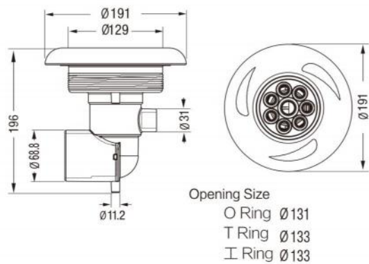
L-2812S 7" Crystal Cyclone Multi-Massage Jet Black
