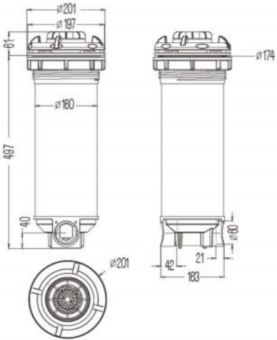
L-2139 Filter Teleweir Assy Low Flow
