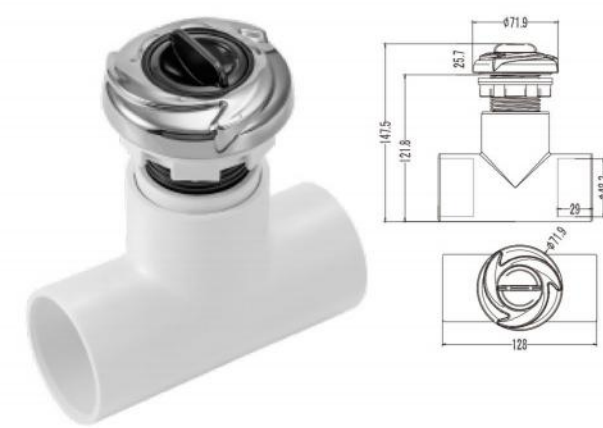
L-2062S 1.5" Cyclone Aromatherapy Canisters Black
