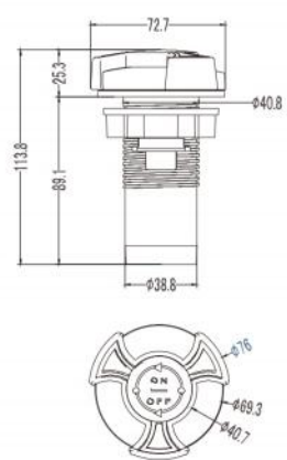
L-2034C 1" Thunder Air Controls Transparent
