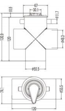
L-2045 1.5" Crystal Diverter Valve Black
