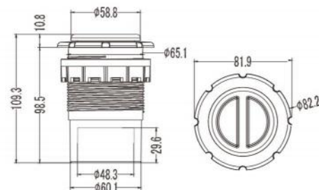
L-2009 1.5" Drain Valve Black
