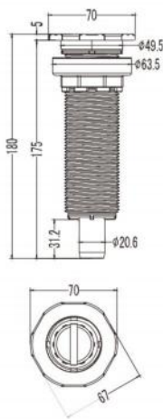
L-2007 1" Drain Valve Black
