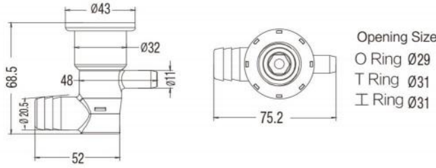
L-0330 1" Jet Body 3/4"RB × 3/8"SB
