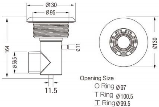
L-1708S 5.5" 7-Holes Directional Jet Black
