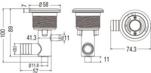
L-0967 2.5" Jet Body 3/4"RB × 3/8"SB
