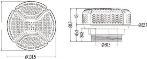
L-3901SA 2" Found Suction
