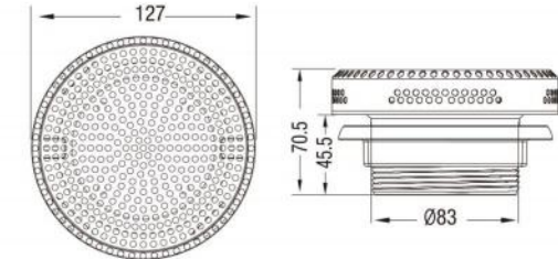
L-3802SA 2" Crystal Thin SS Suction
