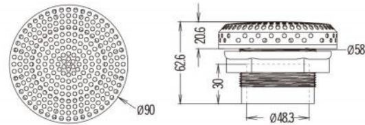
L-3801S 1.5" SS Suction
