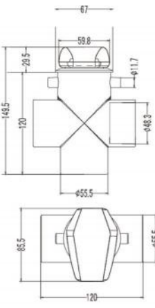
L-2039 1.5" Found Diverter Valve Black
