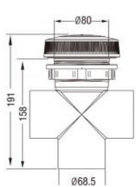
L-7043C 2" Honor Diverter Valve Transparent
