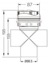
L-7035C 2" Courage Diverter Valve Transparent
