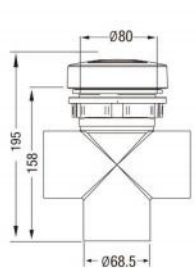
L-2079C 2" Criss-Cross Diverter Valve Transparent
