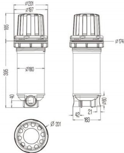
L-2137A Teleweir Skim Filter Low Volume With Protective Cover
