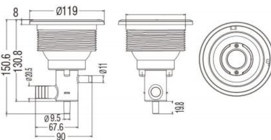
L-0174 5" Jet Body 3/4"RB × 3/8"SB
