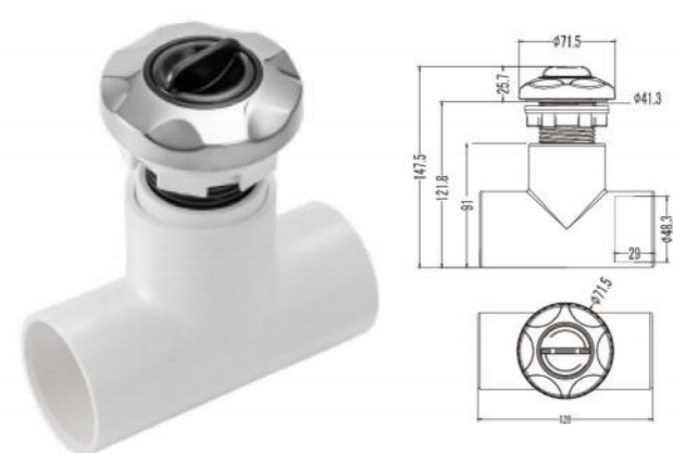
L-2061S 1.5" Louts Aromatherapy Canisters Black
