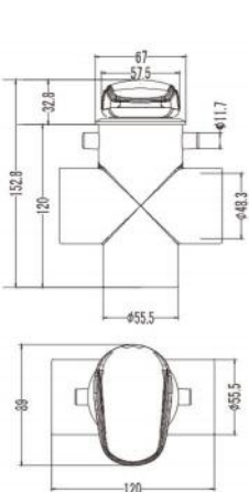
L-2044 1.5" Flying Diverter Valve Black
