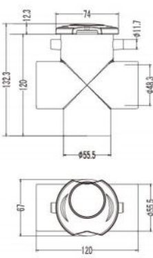
L-2048 1.5" Luxury Elegant Diverter Values Black
