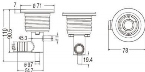
L-0046 3" Jet Body 3/4"RB × 3/8"SB
