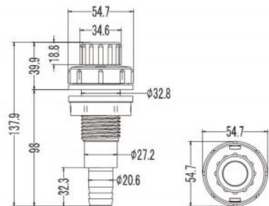
L-2008 3/4" Drain Valve Black
