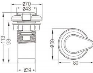
L-2247C 1" Elegant Air Controls Transparent
