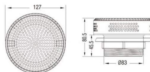
L-3802SB 2" Crystal Thick SS Suction
