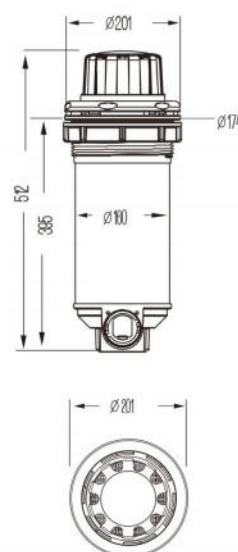
L-2125A Teleweir Skim Filter Low Volume
