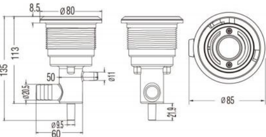
L-0310 3.5" Jet Body 3/4"RB × 3/8"SB
