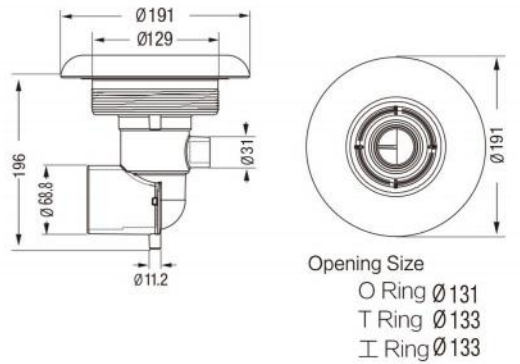
L-2801S 7" Crystal Directional Jet Black
