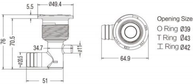
L-0015 2" Jet Body 3/4"RB × 3/8"SB
