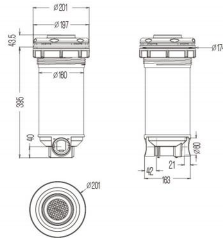
L-2136A Teleweir Skim Filter
