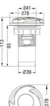
L-2032S 1" Xiongfeng Air Controls (SS Cover)
