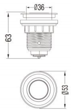
L-2904K Chrome-plated Air Control
